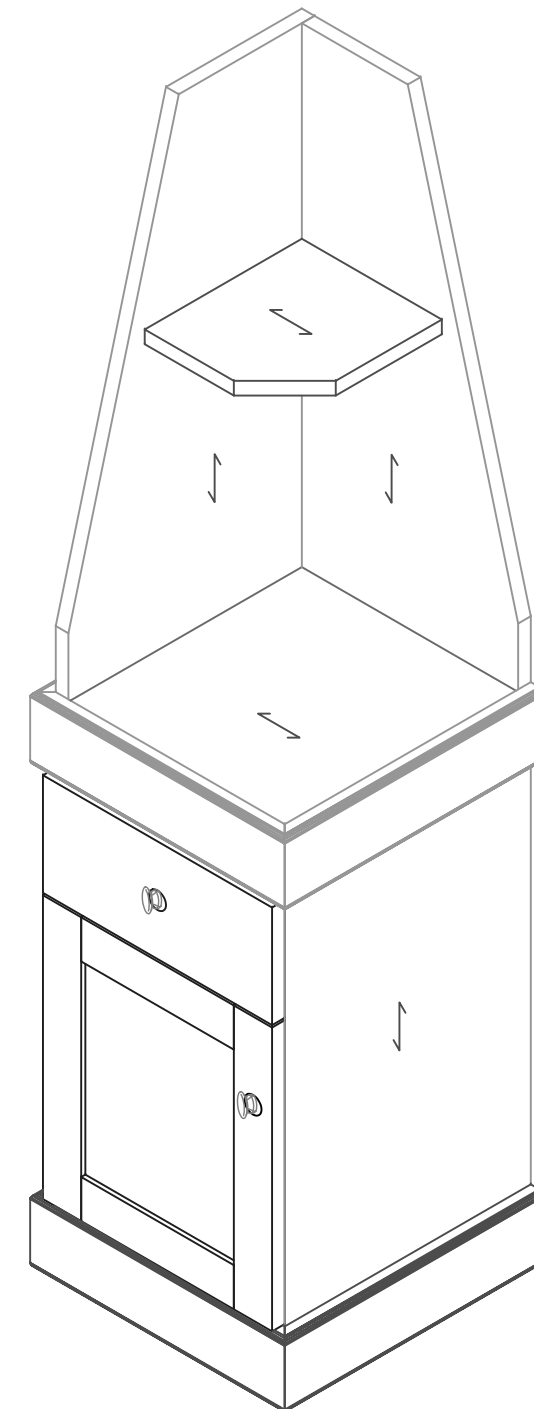
CABINET WITH BOOKSHELF ISOMETRIC: NTS
